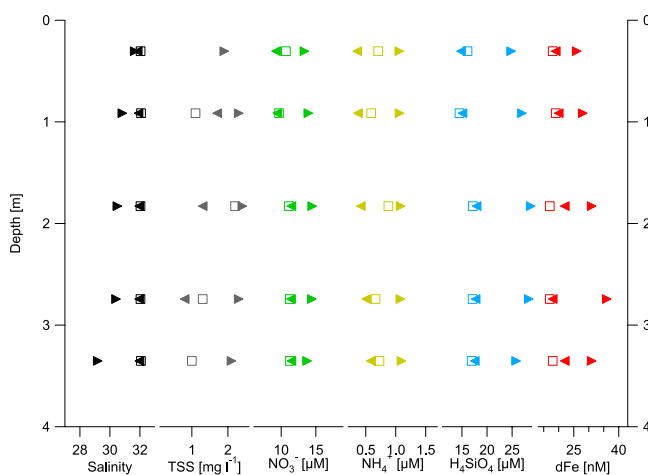
Figure 4. Chemical properties at the mouth of Alsea Bay, OR, 12 January 2005. Samples were collected at ebb tide (right-facing triangles), flood tide (left-facing triangles), and high tide (squares).
