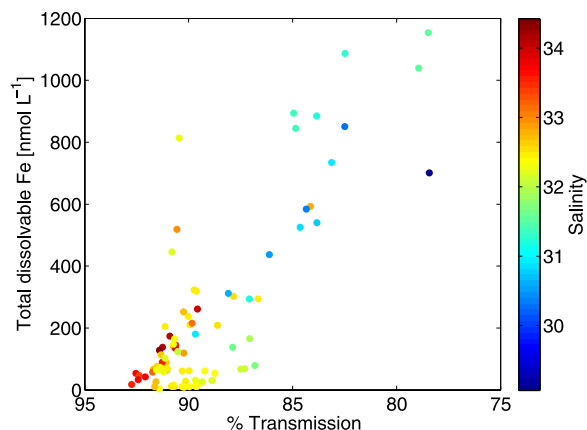
Figure 3. Relationship between total dissolvable Fe concentration and light transmission for samples collected in winter 2003 on the OR shelf. Samples are color-coded by salinity.
